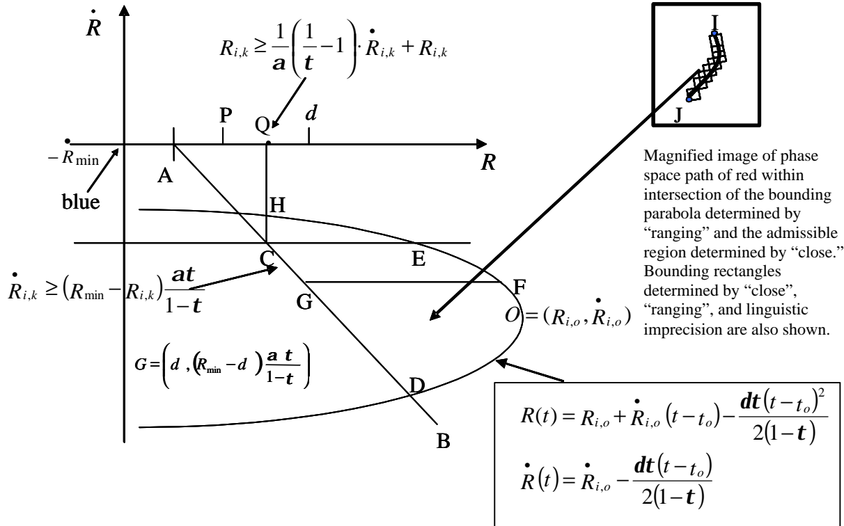
Figure 1: Trajectories within the combined admissible region of phase space determined by "close" and "ranging."
