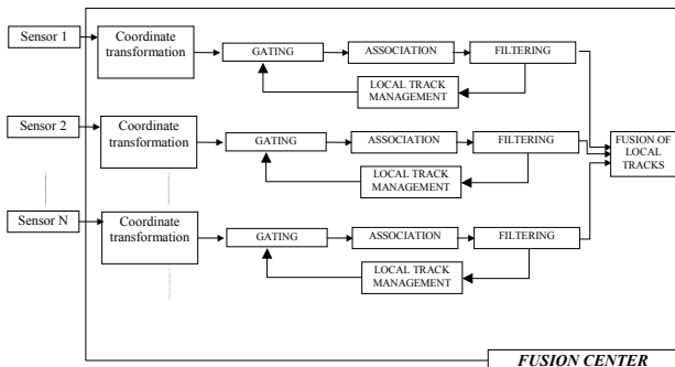
Fig. 4. Distributed architecture
