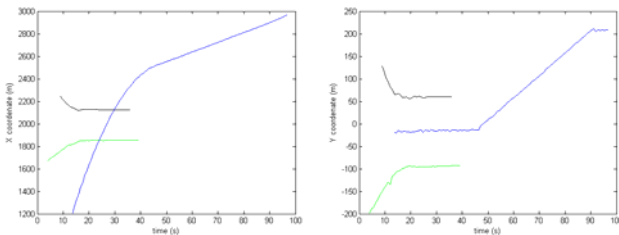
Fig. 9. Aircraft X and Y coordinates in scenario 3.
